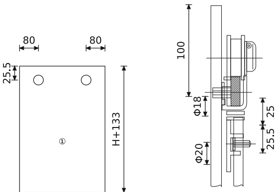
30X10 方管截面安装图 Sectional Installation Map with 30*10 Square Pipe
