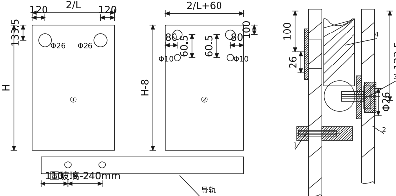
Φ25 管浴室吊轮截面安装图 Sectional Installation Of Φ25 Pipe Bathroom Hanging Wheel
