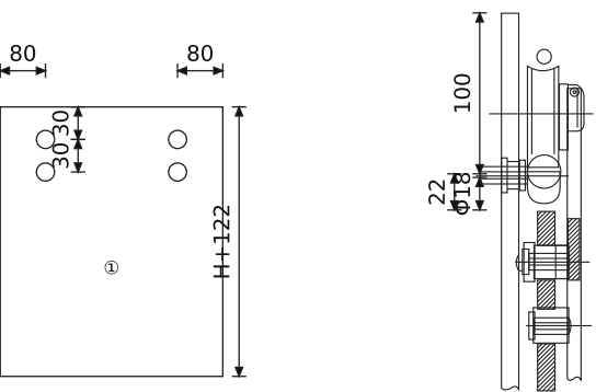
Φ25 管浴室吊轮截面安装图 Sectional Installation Of Φ25 Pipe Bathroom Hanging Wheel
