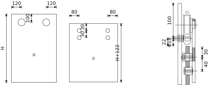
Φ25 管浴室吊轮截面安装图 Sectional Installation Of Φ25 Pipe Bathroom Hanging Wheel
