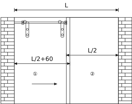
Φ25 管浴室吊轮平面安装图 Installation of Φ25 pipe bathroom hanging wheel
