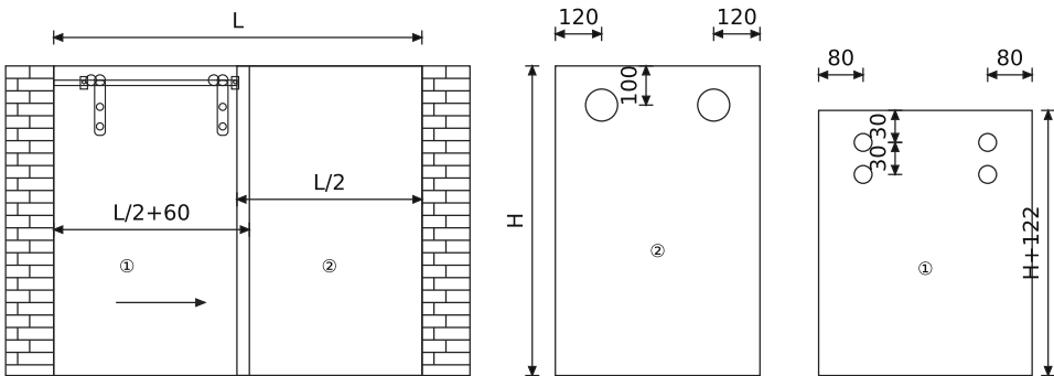
Φ25 管浴室吊轮平面安装图 Installation of Φ25 pipe bathroom hanging wheel
