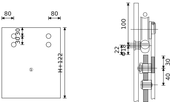
Φ25 管浴室吊轮截面安装图 Sectional Installation Of Φ25 Pipe Bathroom Hanging Wheel
