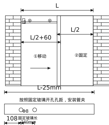
30X10 方管带防跳平面安装图 30X10 installation of square pipe with jumping-proof pillar
