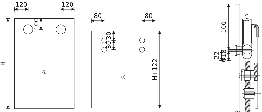
Φ25 管浴室吊轮截面安装图 Sectional Installation Of Φ25 Pipe Bathroom Hanging Wheel
