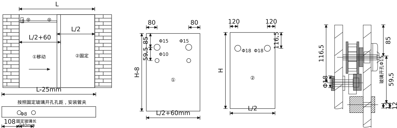
30X10 方管带防跳平面安装图 30X10 installation of square pipe with jumping-proof pillar
