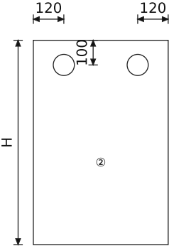
Φ25 管浴室吊轮平面安装图 Installation of Φ25 pipe bathroom hanging wheel
