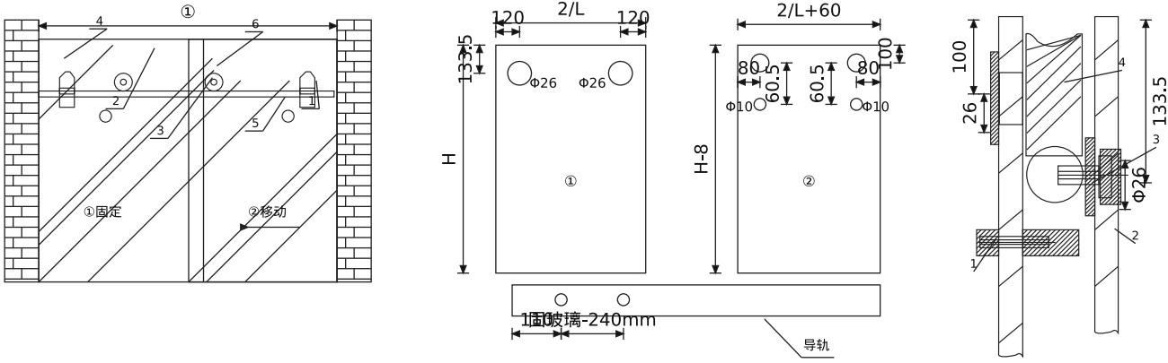
Φ25 管浴室吊轮平面安装图 Installation of Φ25 pipe bathroom hanging wheel
