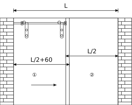
Φ25 管浴室吊轮平面安装图 Installation of Φ25 pipe bathroom hanging wheel
