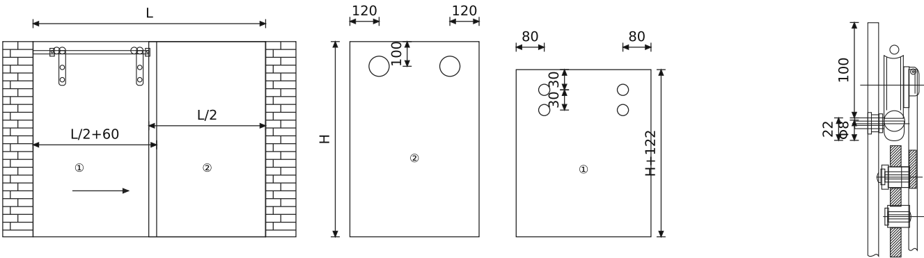
Φ25 管浴室吊轮平面安装图 Installation of Φ25 pipe bathroom hanging wheel
