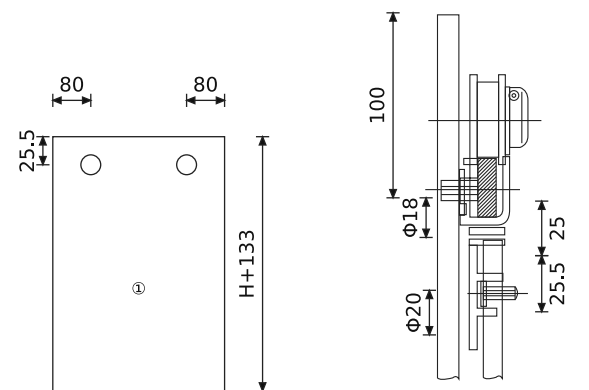
30X10 方管截面安装图 Sectional Installation Map with 30*10 Square Pipe
