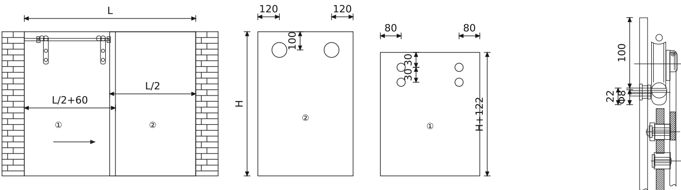
Φ25 管浴室吊轮平面安装图 Installation of Φ25 pipe bathroom hanging wheel
